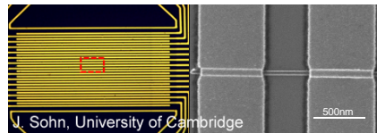
A memory device built around a single zinc oxide nanowire. Each nanowire is less than 100 nm in diameter.
